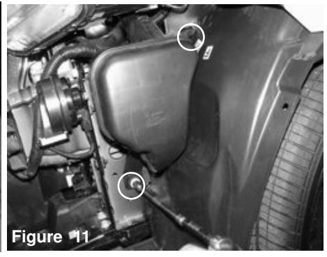
Figure 11 Loosen the 2 screws holding in the resonator box.
