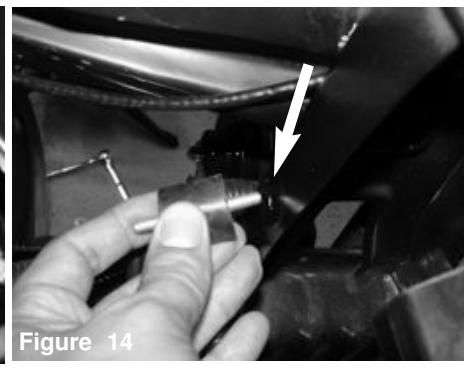
Figure 14 Now install the vibra mount to the hole
