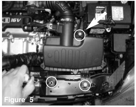
Figure 5 With 10mm socket and ratchet, loosen the 3 screws holding in the stock air box.
